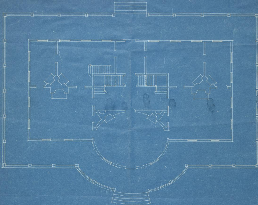
First Floor Plan. General Knox Mansion 50 Thomaston, Me
